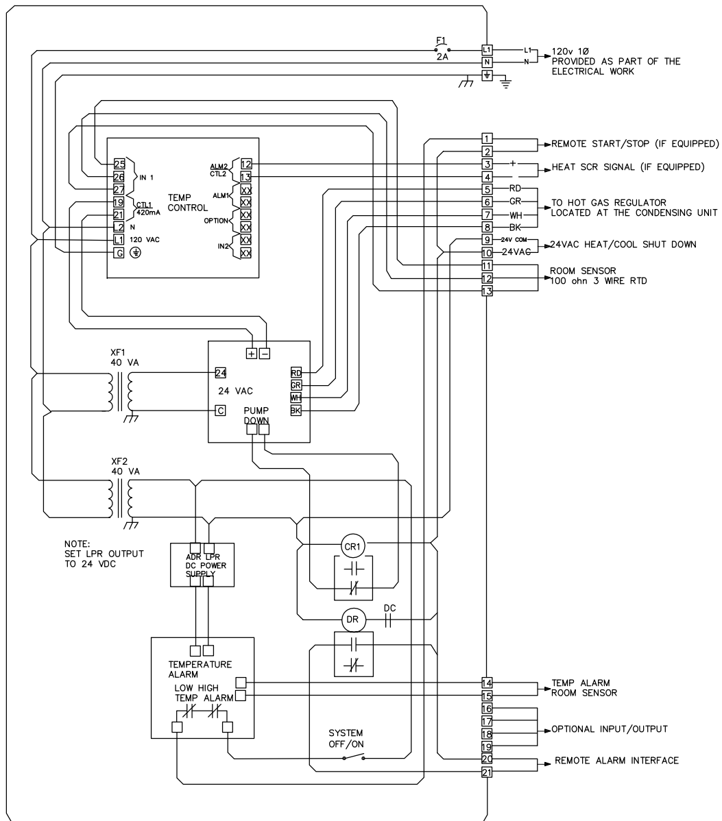
PANEL WIRING SCHEMATIC
