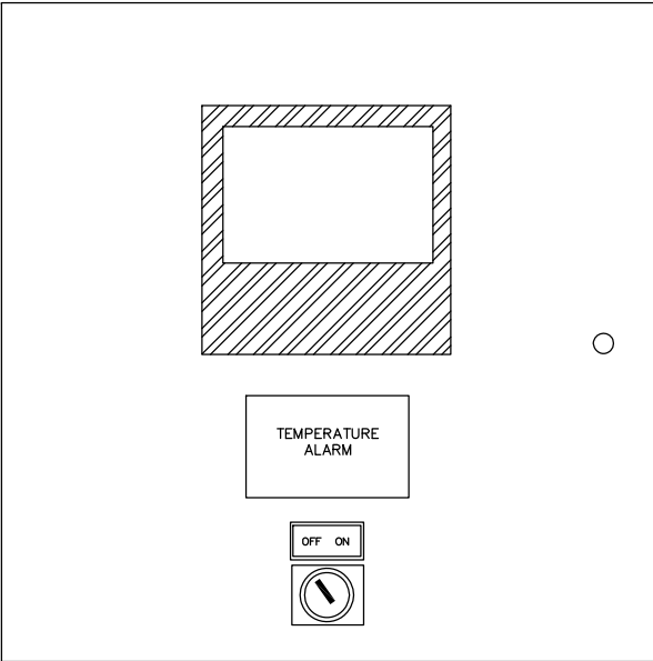
FRONT PANEL LAYOUT
