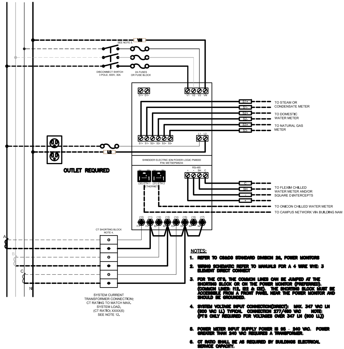
E-03: STANDARD ION PM8000 SERIES ELECTRIC METER DRAWING - ION METER WIRING
