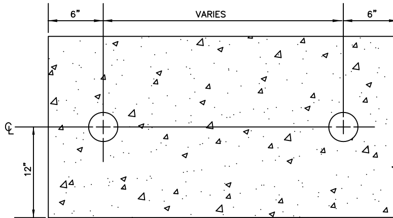
TOP VIEW OF SLAB
